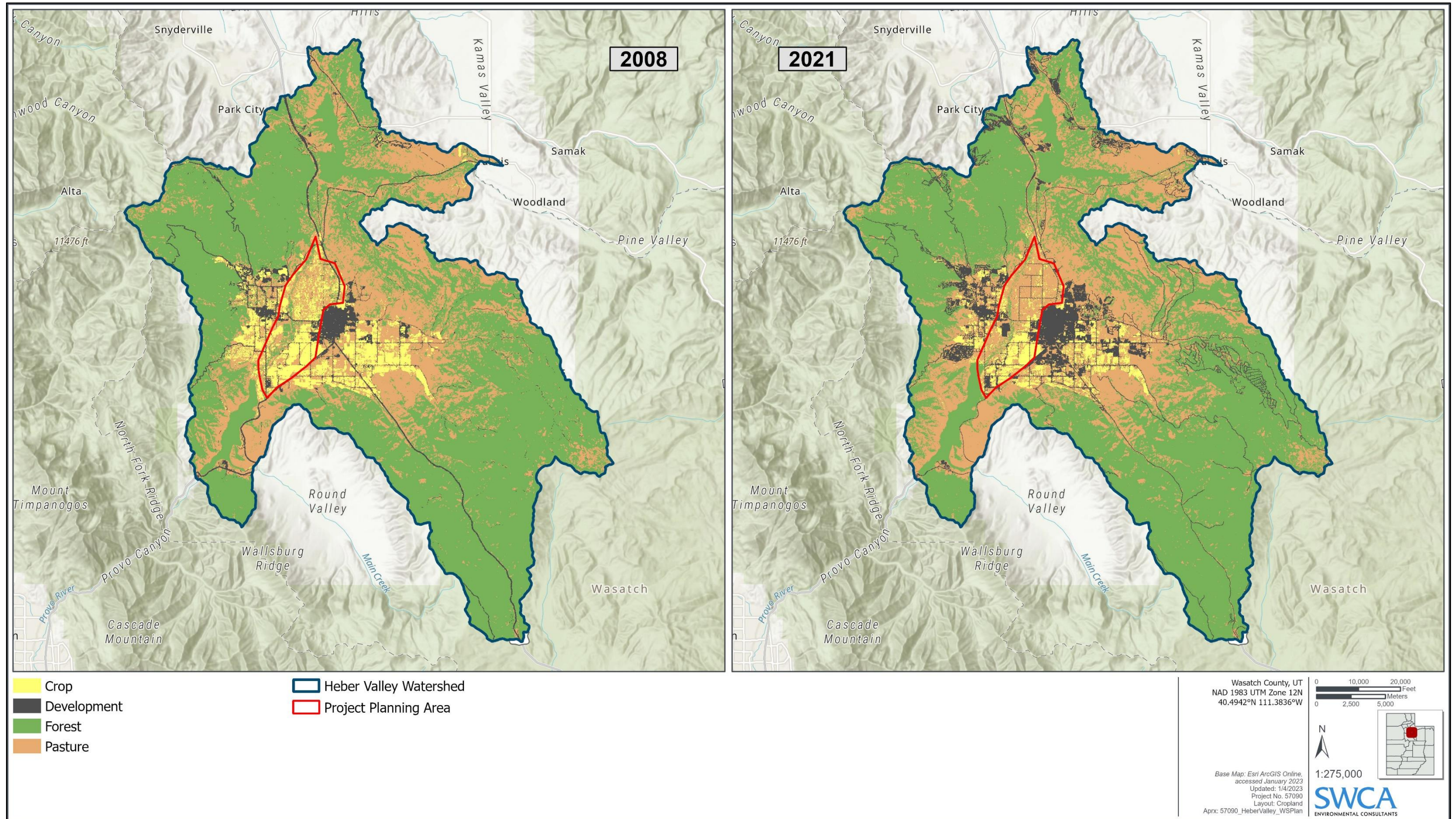
Figure 4. Cropland Data Layer data in the Heber Valley watershed.
