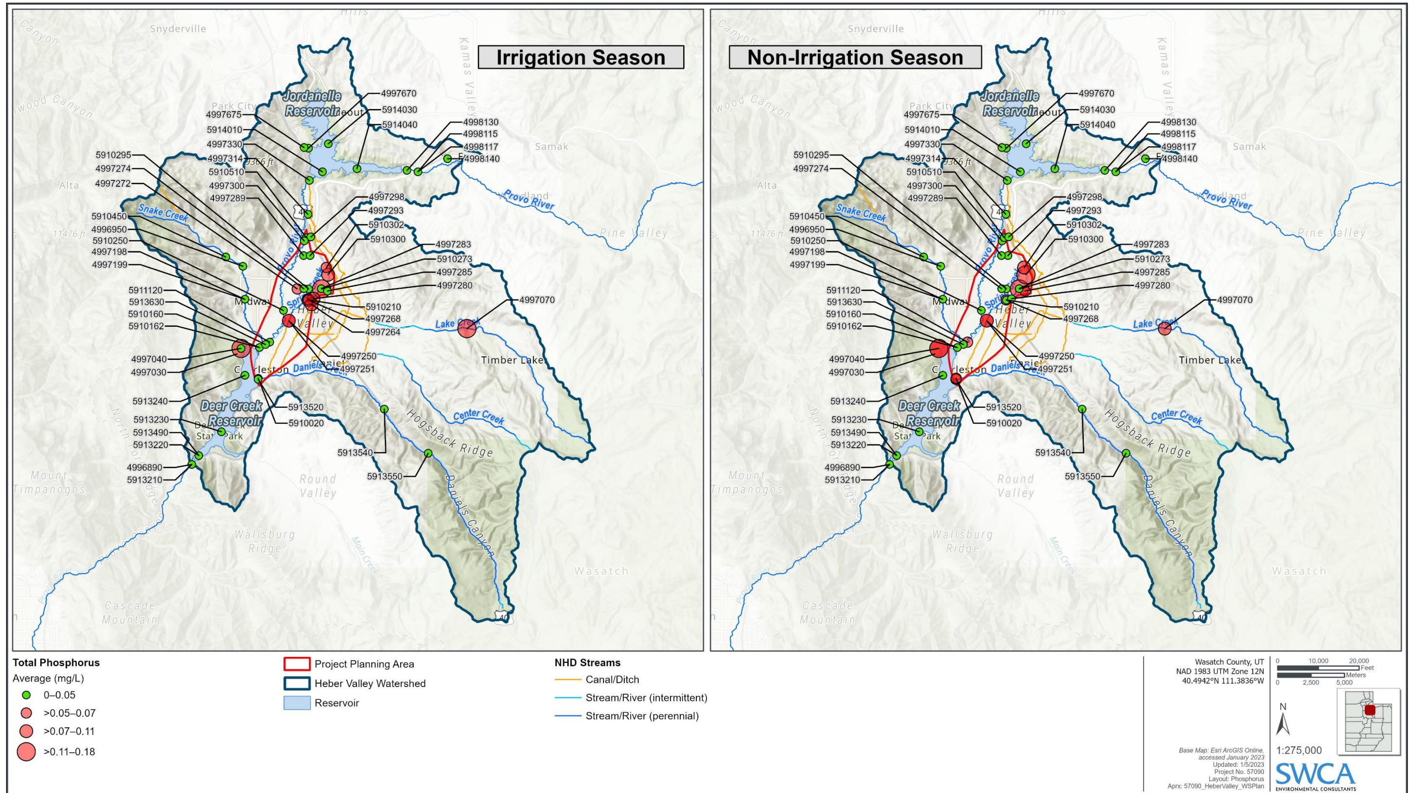
Figure 18. Utah Division of Water Quality monitoring locations in the Heber Valley watershed and mean total phosphorus concentrations between 2001 and 2021.
