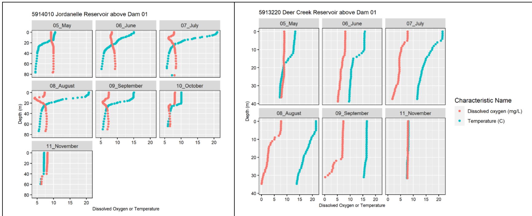
Figure 20. Depth profiles for temperature and dissolved oxygen at Jordanelle Reservoir (left) and Deer Creek Reservoir (right) in 2020.
